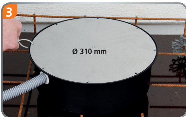
Insert the concrete pipes and fix the cover on the Light-box with the included accessories.
