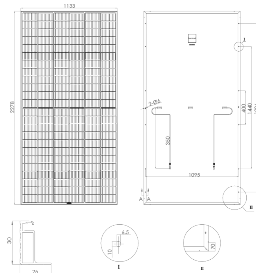
Fig. 1: External dimensions (in mm) and components for SR-72MHLPRO
