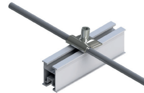
Attach the aluminium wire with a wire clamp
