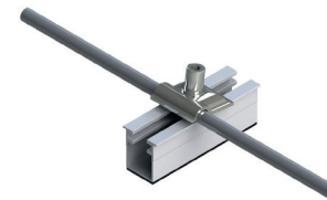
Attaching the aluminium wire with a wire clamp
