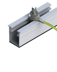
Attaching the earthing wire with an anchor bolt
